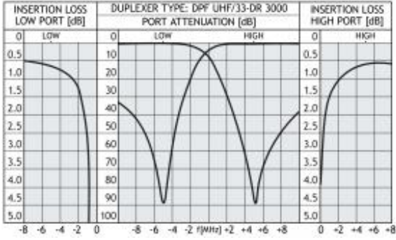
MOUNTING IN MOTOROLA DR 3000
